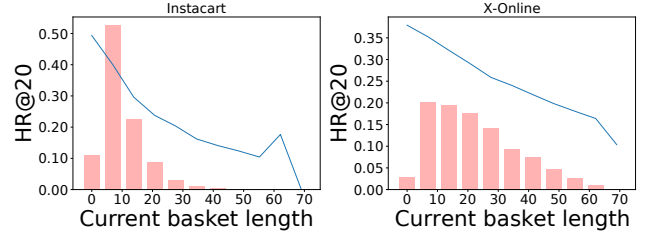
Figure 2: Performance of PerNIR in terms of \text{HR@20} based on the number of items in the current basket. Bars show the distribution of basket lengths.
