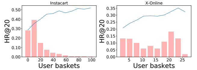
Figure 3: Performance of PerNIR in terms of \text{HR@20} based on the number of baskets in users' history. Bars show the distribution of number of baskets per user.
