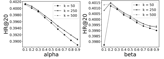
Figure 1: Sensitivity of the performance in terms of \text{HR@20} to hyper-parameters \alpha and \beta for different values of k on Instacart.
